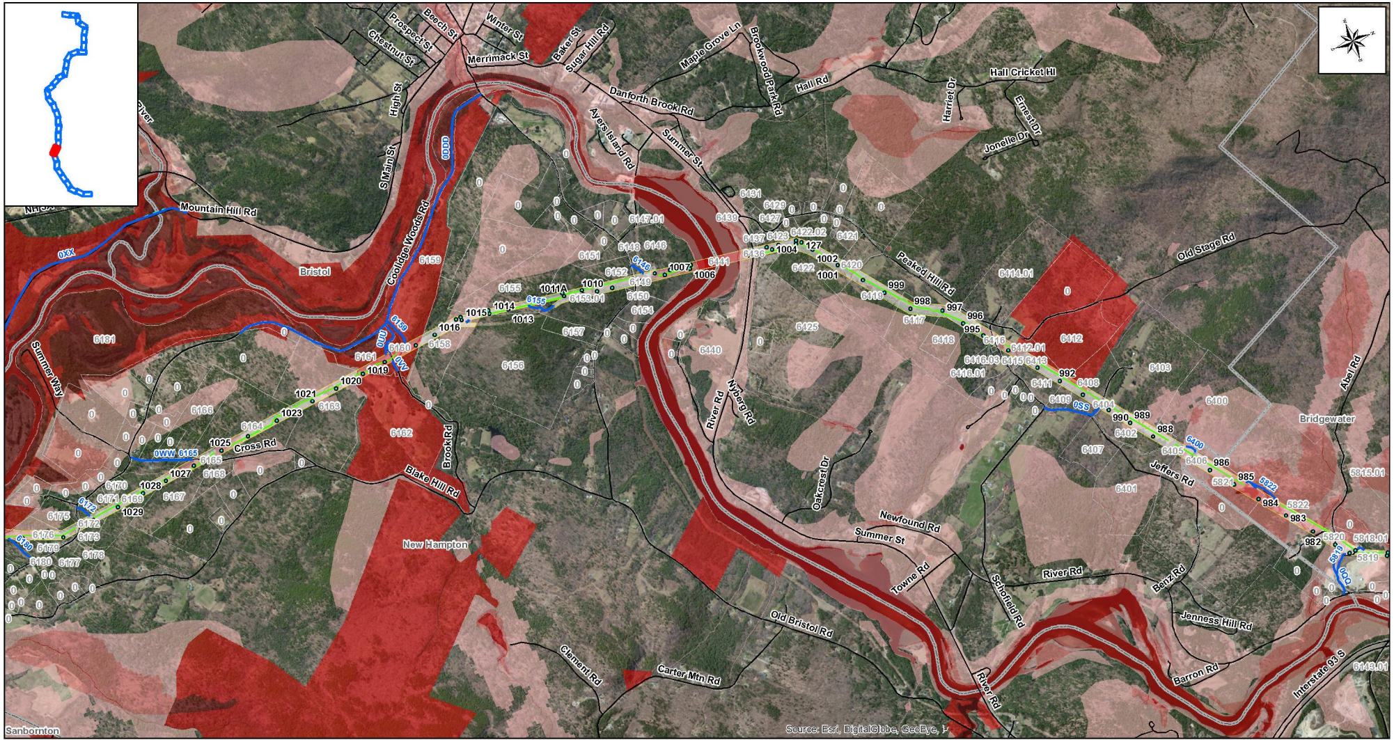
HVDC Risk Assessment Model In-ROW and Off-ROW Map 9 of 32 February 1, 2012
