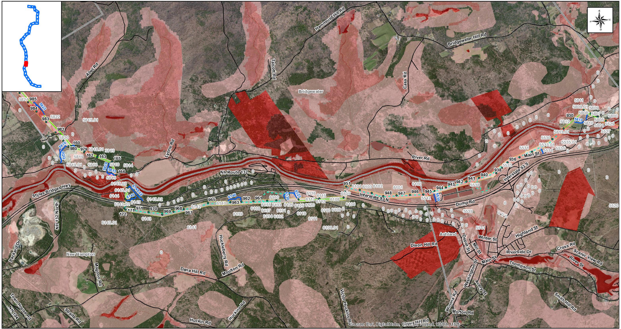
HVDC Risk Assessment Model In-ROW and Off-ROW Map 10 of 32 February 1, 2012
