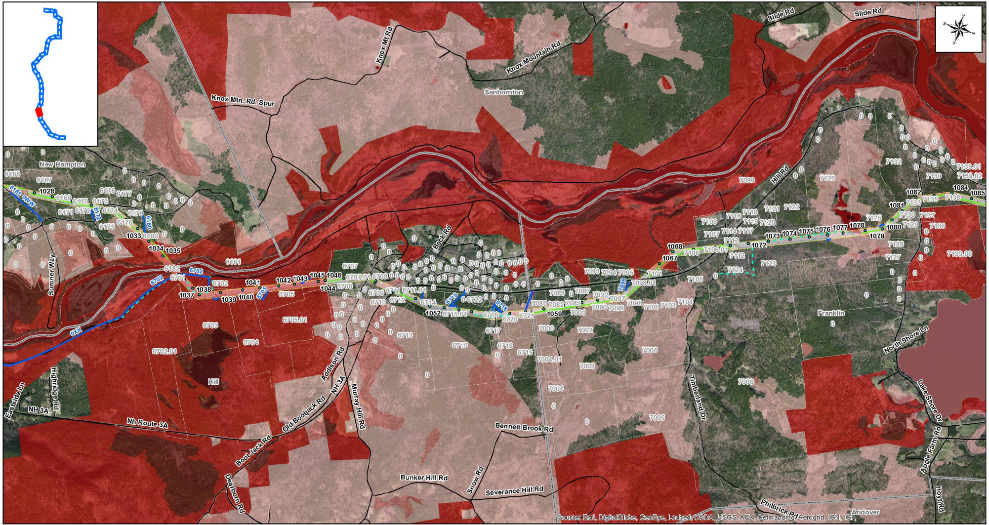
HVDC Risk Assessment Model In-ROW and Off-ROW Map 8 of 32 February 1, 2012
