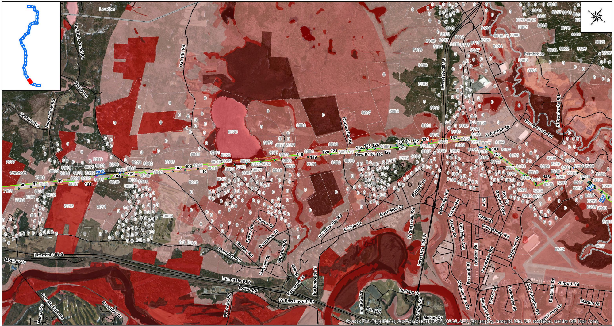
HVDC Risk Assessment Model In-ROW and Off-ROW Map 4 of 32 February 1, 2012
